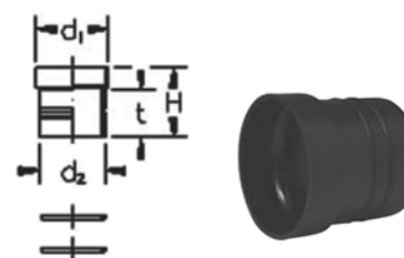
Adaptors to PVC
