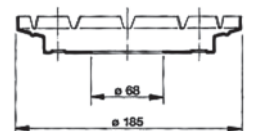
Fixing ring
