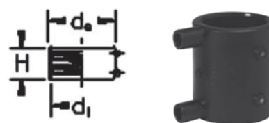
Electro-fusion coupler
