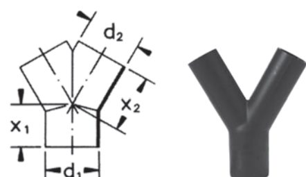
Y-branch 30°
