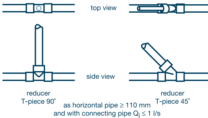
Illus.3.7 Top connection.
