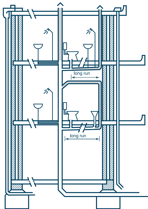
Illus. 2.3 Example of restricted secondary discharge system.
