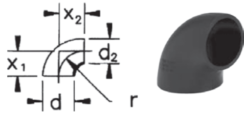
Reduced elbow 90°
