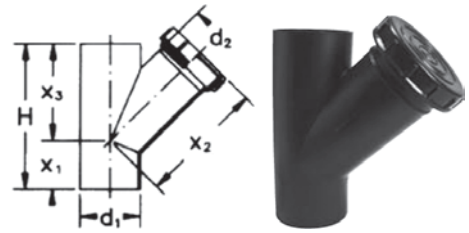
Access fitting 45°
