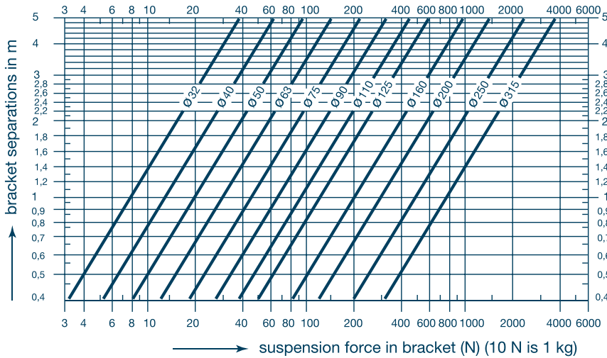
Illus. 7.1 Relationship between bracket separations, pipe diameter and suspension forces with filled HDPE pipework.
