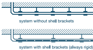
7.8 System without/with shell brackets.
