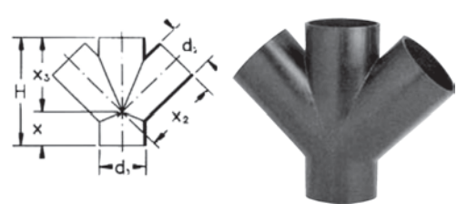
Double branch 45°
