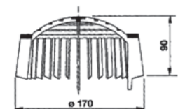
Protection cap, aluminium
