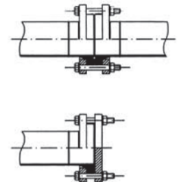
Flange connections
