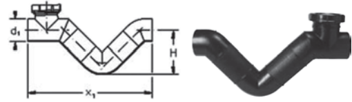
Outlet connectors
