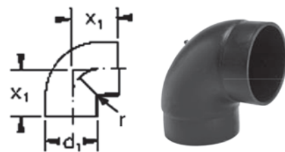
Elbow 88 1/2°
