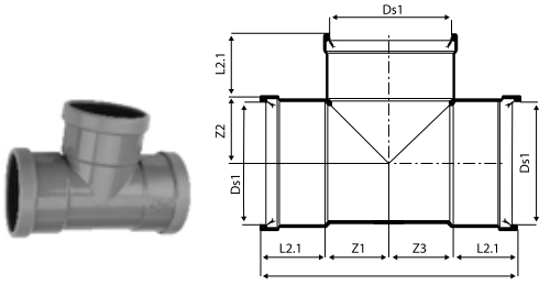
Tee 88° (3 Socket)
