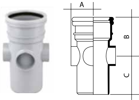
Unequal Branch (3 way bossed pipe. All bosses molded solid)
