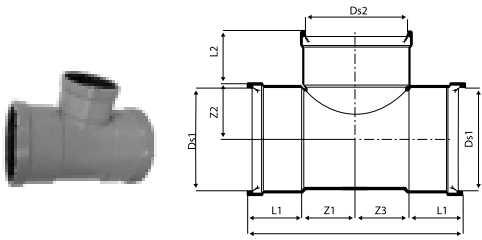
Reducing Tee 88° (3 Socket)
